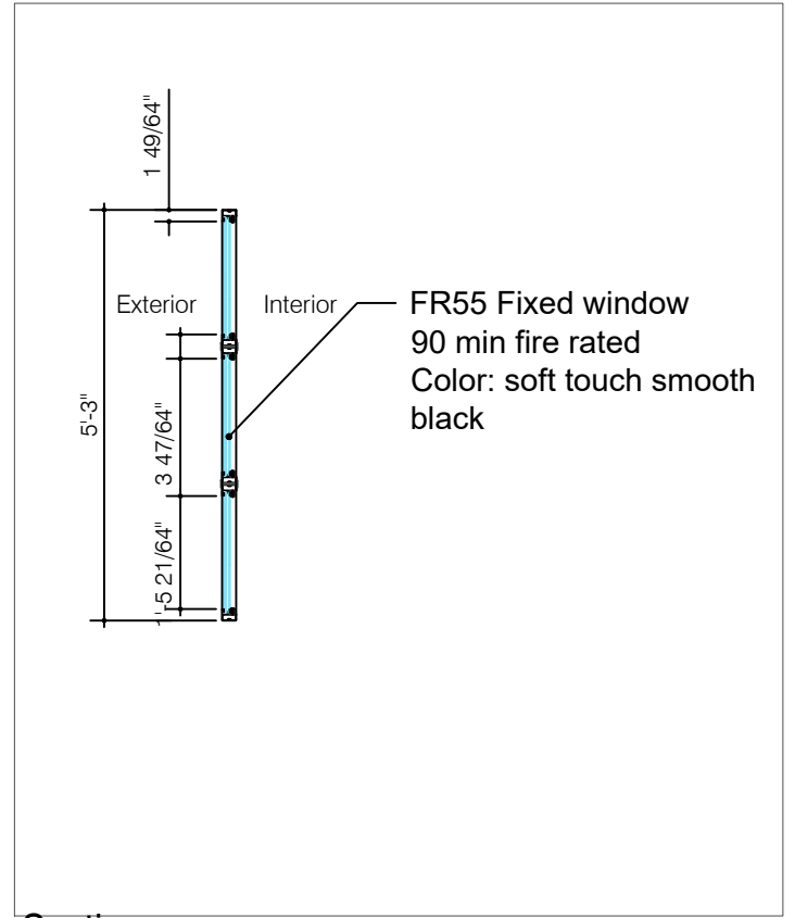
Section
