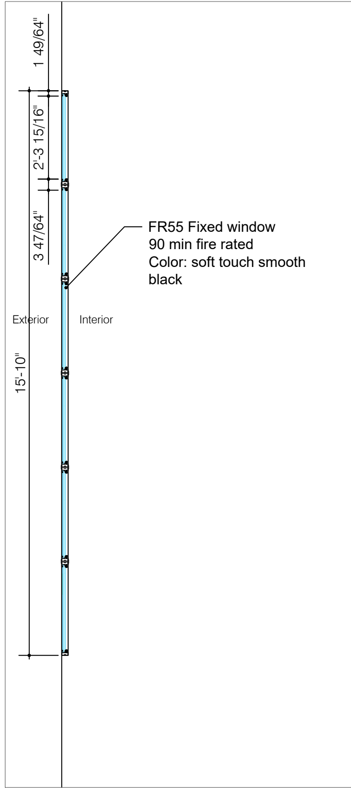
Section
