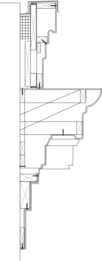
PROPOSED CORNICE SECTION DETAIL
