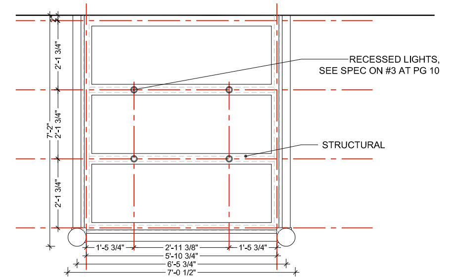
ENLARGED REFLECTED CEILING PLAN - PROPOSED
