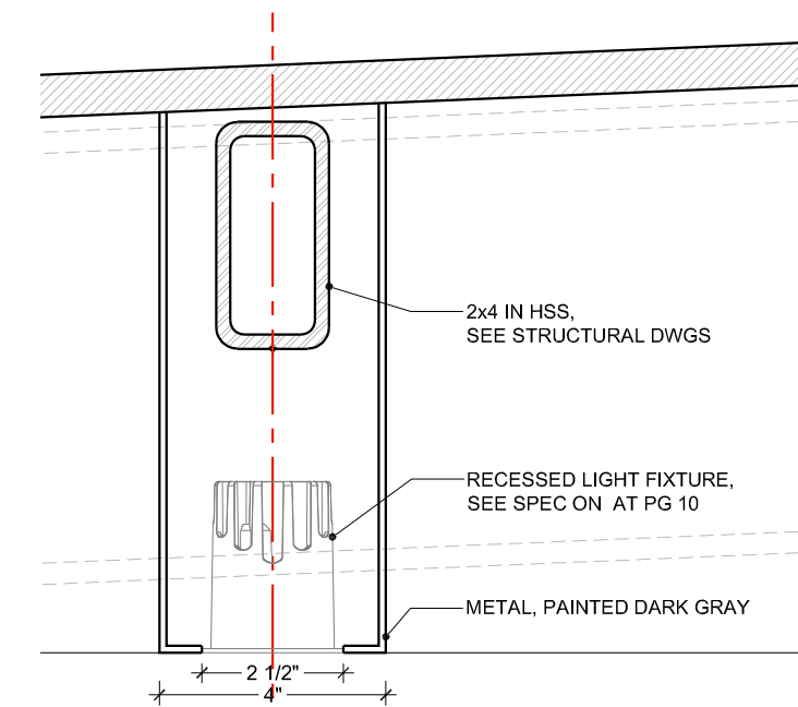
MARQUEE DETAIL - LIGHTING
