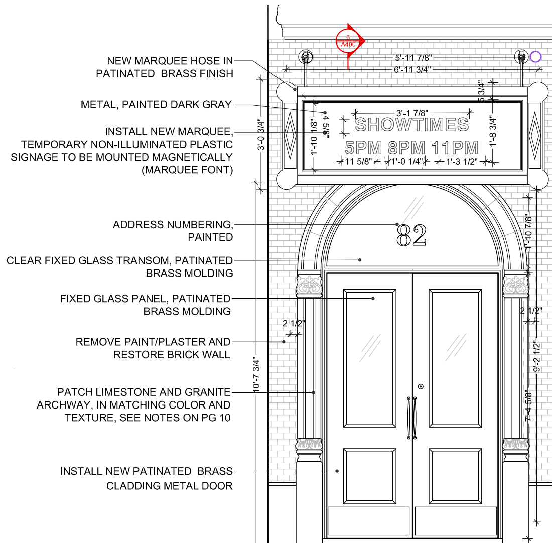
FRONT ELEVATION - PROPOSED
