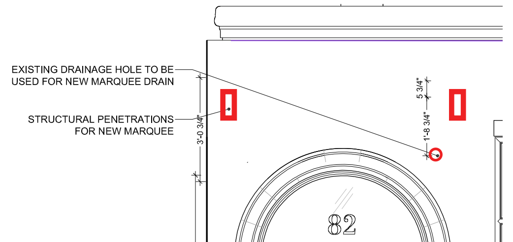
ENLARGED FRONT ELEVATION - PROPOSED
