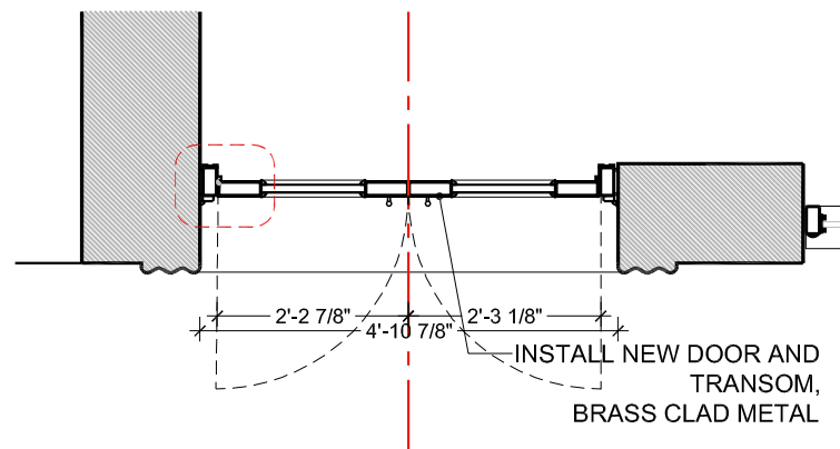
ENLARGED PLAN - PROPOSED
