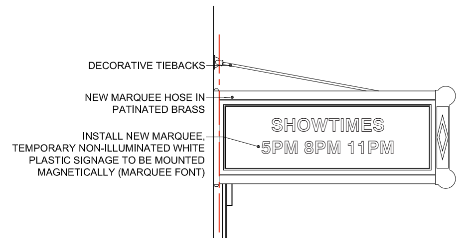
ENLARGED SIDE ELEVATION - PROPOSED
