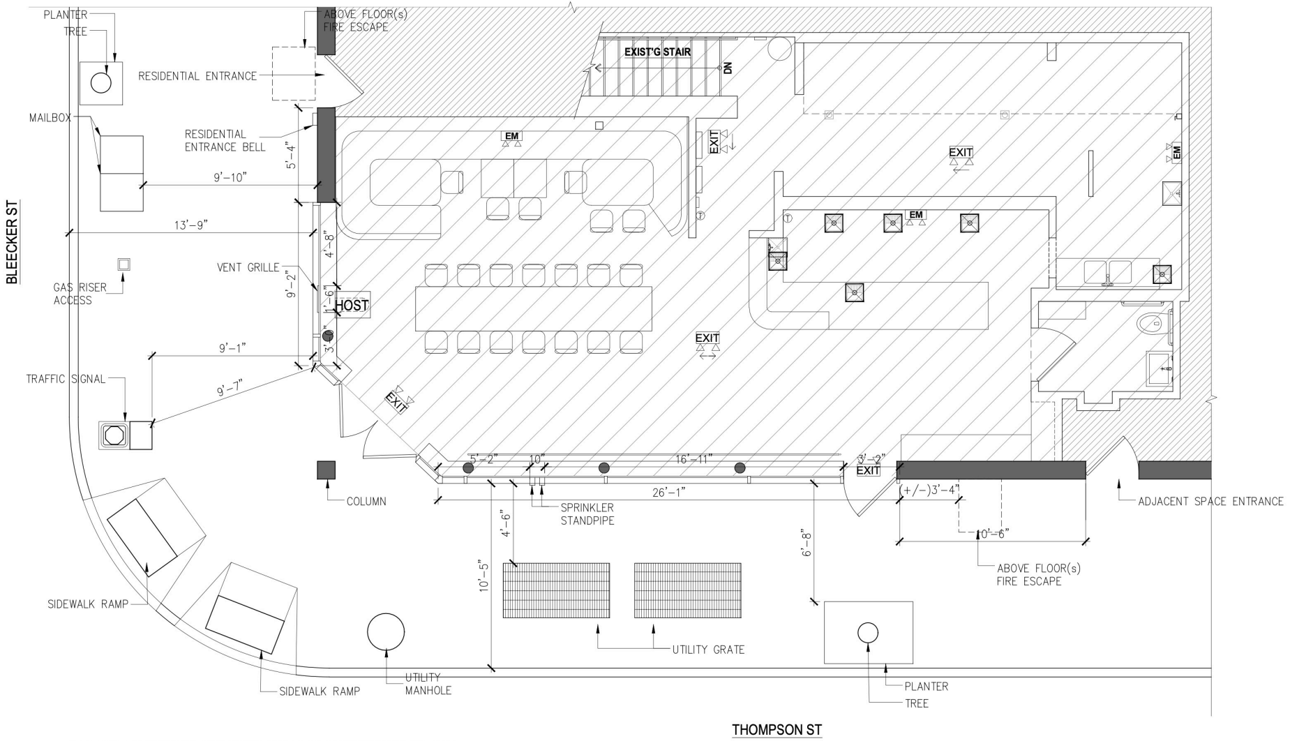
0 155 BLEECKER ST SIDEWALK EXISTING PLAN N.T.S.
