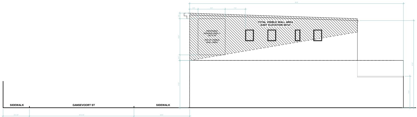
EAST ELEVATION
