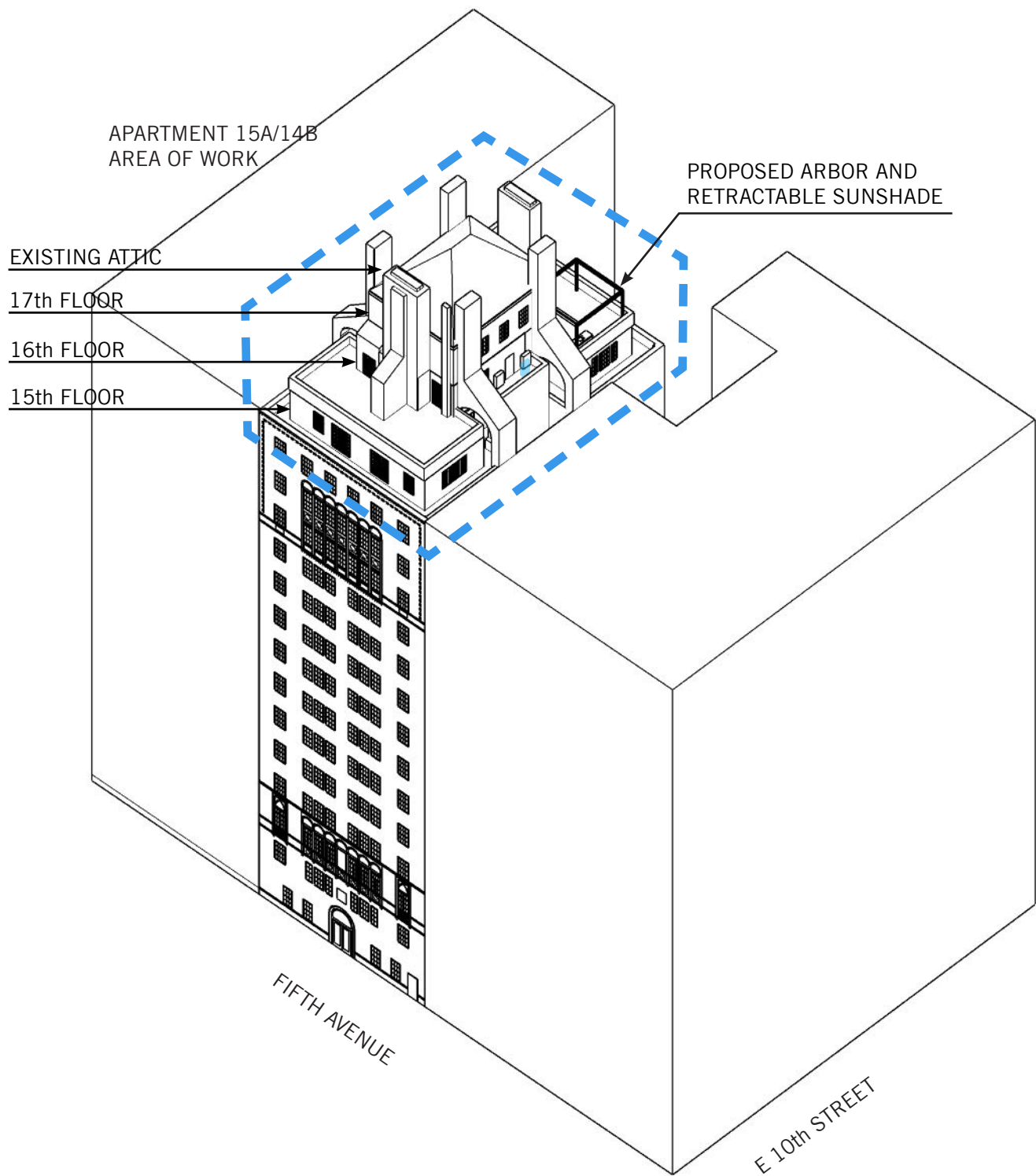
AXONOMETRIC VIEW
