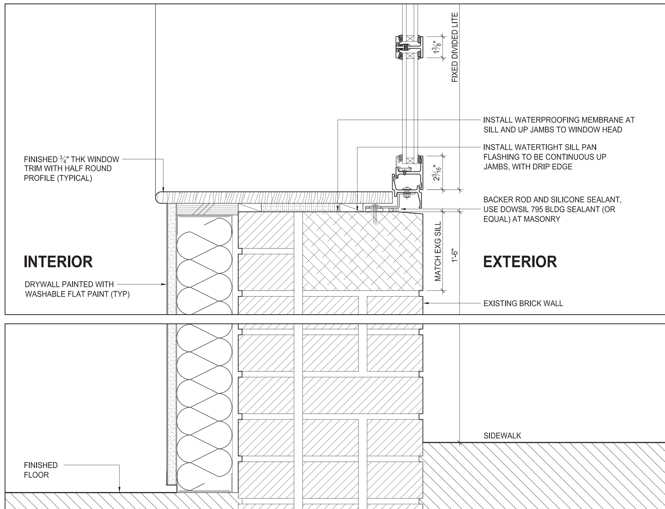
WINDOW DETAIL: SILL OPERABLE WINDOW
