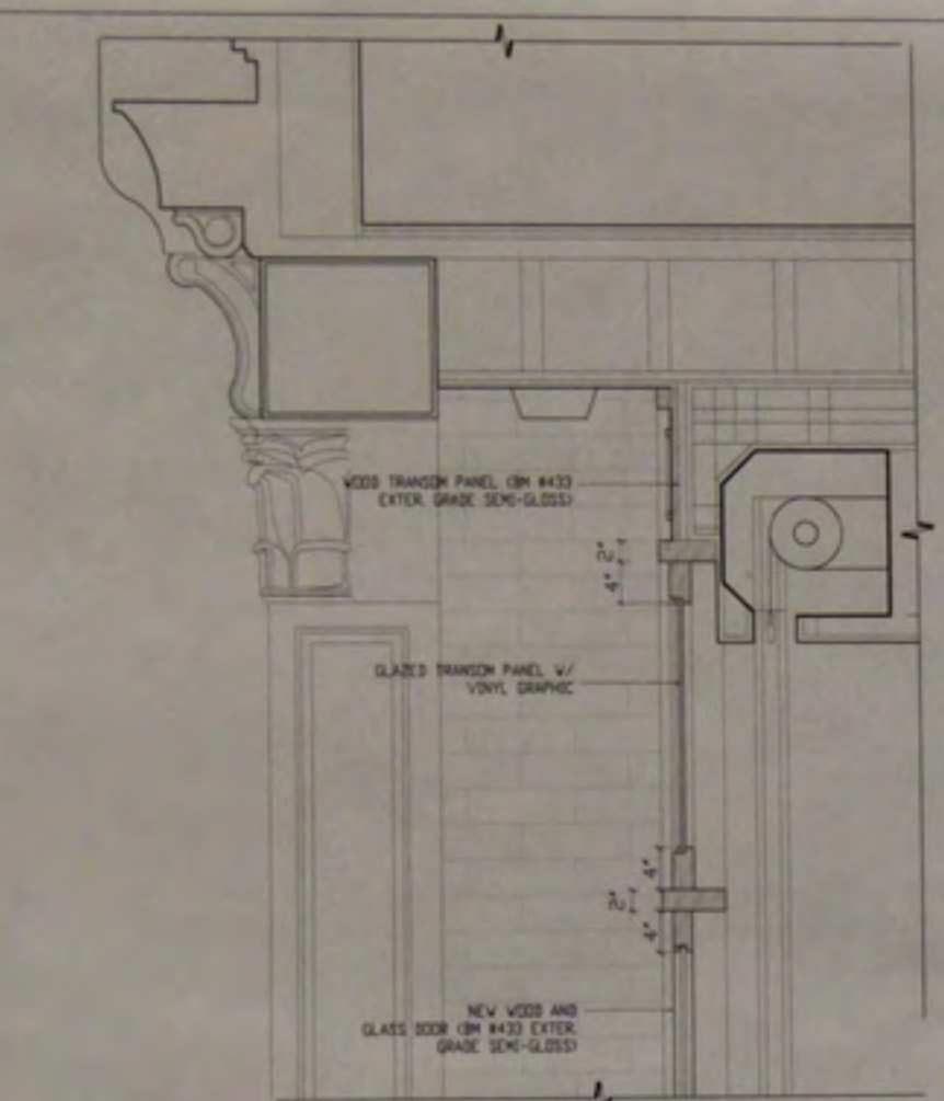
02 SECTION DETAIL AT DOOR ALCOVE SCALE 1/2" = 1'-0"
