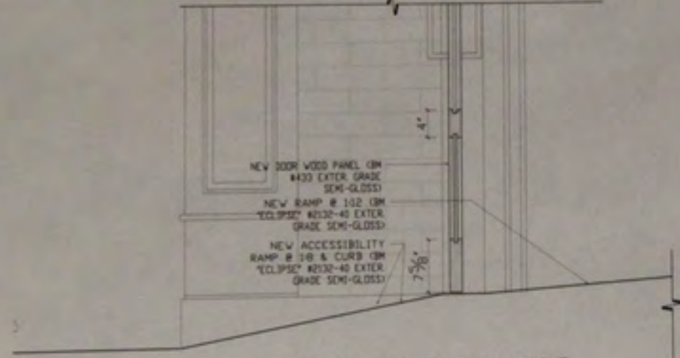
01 SECTION DETAIL AT DOOR ALCOVE SCALE 1/2" = 1'-0"
