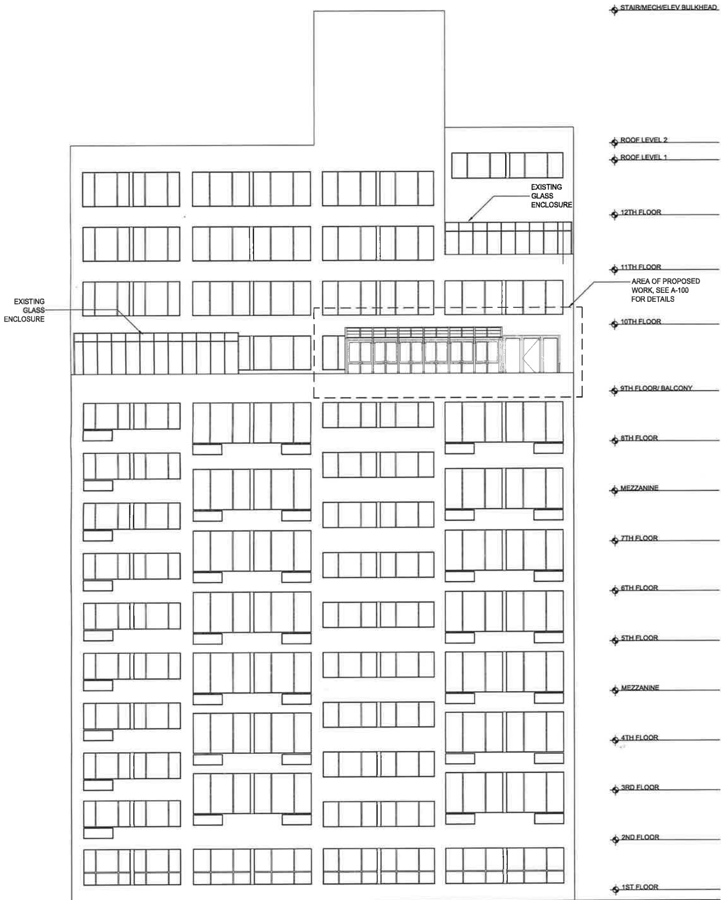
A 77 BLEECKER STREET SCHEMATIC BUILDING ELEVATION SCALE : 1/8" = 1'-0"
