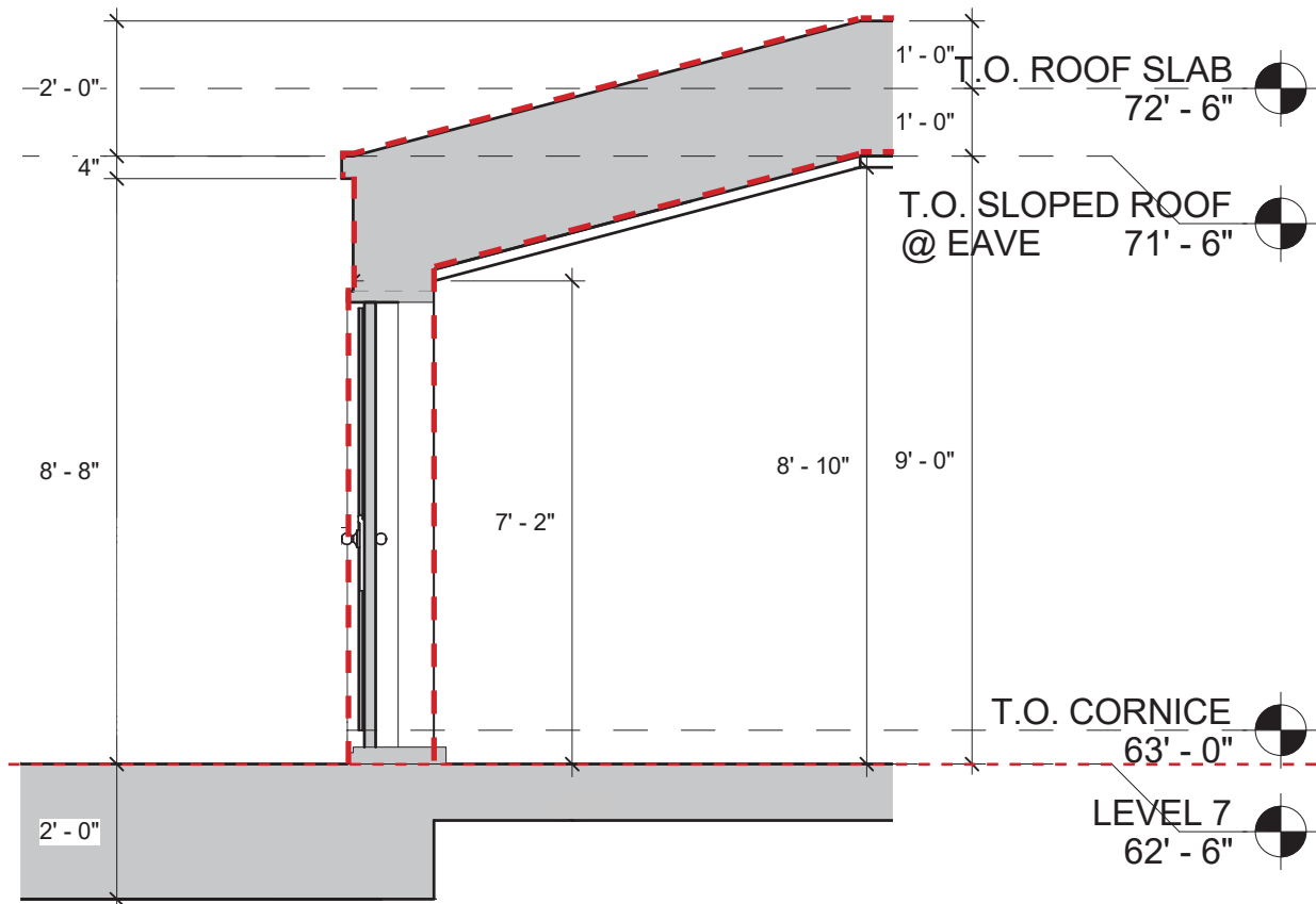
WEST WALL SECTION (APPROVED WITH CONDITIONS - FEBRUARY 6, 2018 PUBLIC MEETING)
