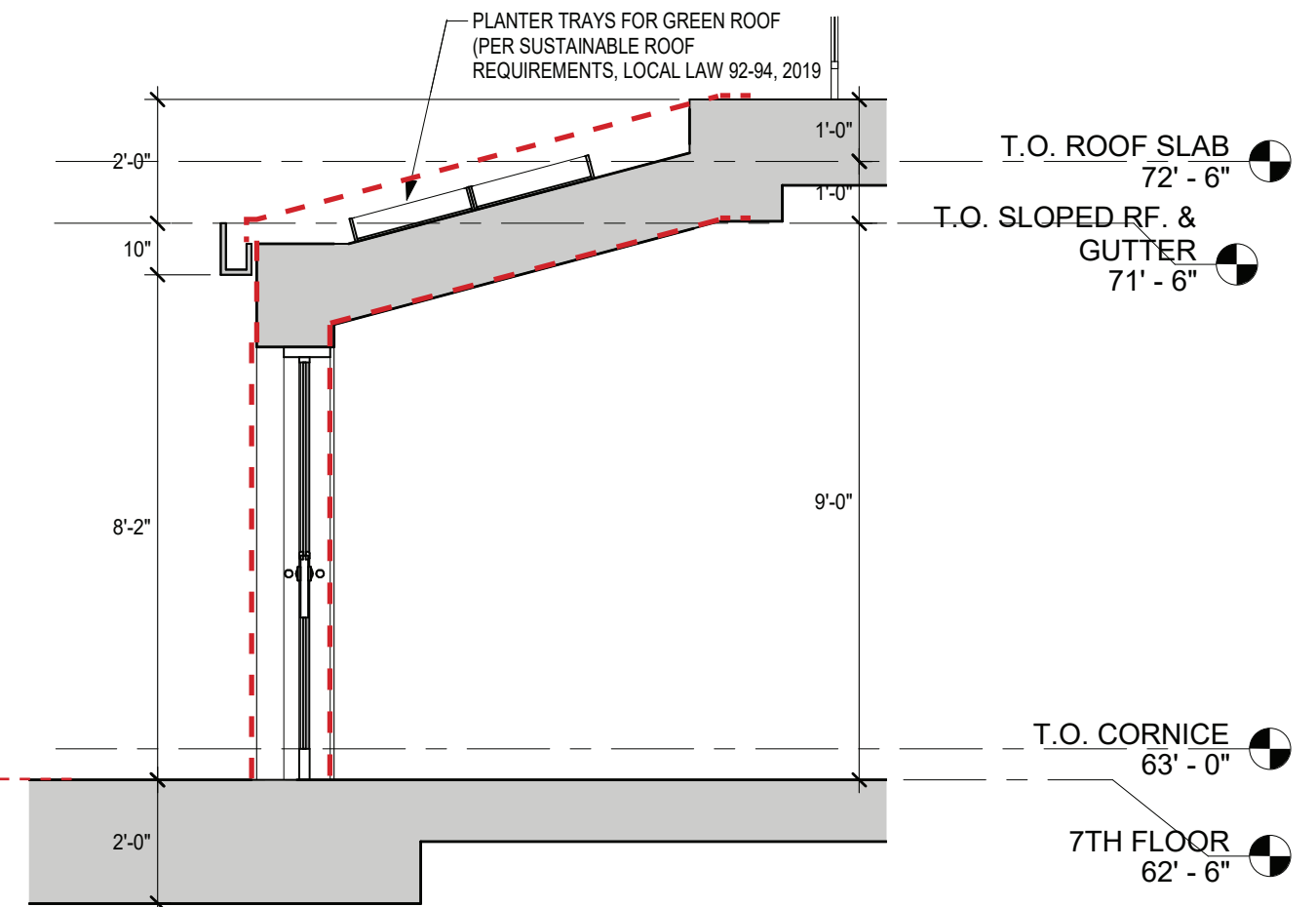
WEST WALL SECTION (PROPOSED - NOVEMBER 2020)
