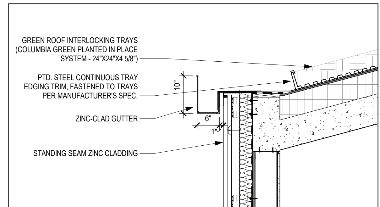
PROPOSED DETAIL AT GUTTER / ROOF EDGE
